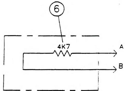
WIRING DETAIL
